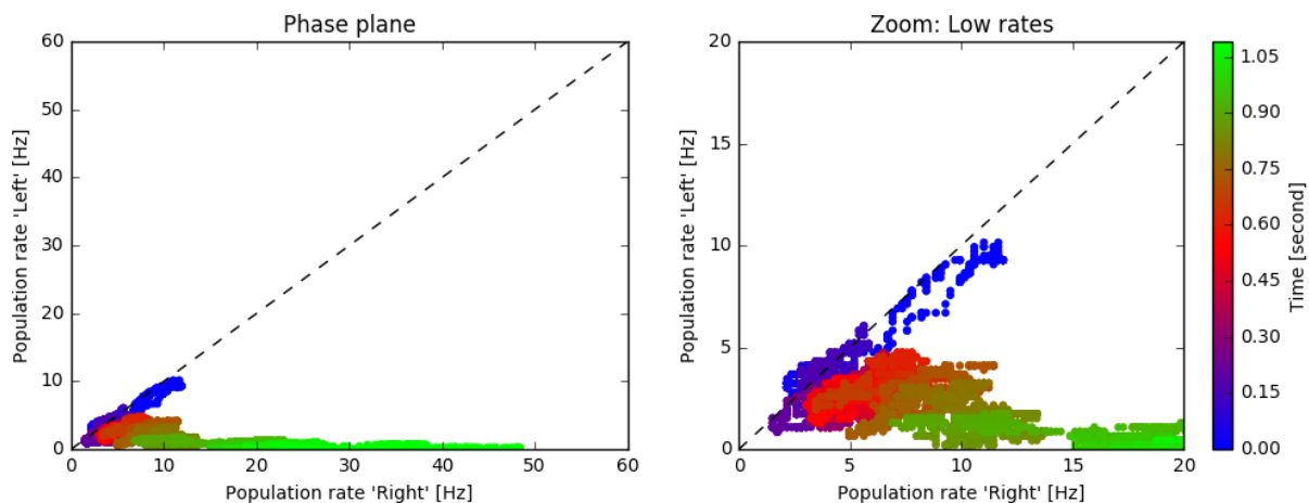
Fig. 18: Decision Space. Each point represents the firing rates of the two subpopulations “Left” and “Right” at a given point in time (averaged over a short time window). The color encodes time. In this example, the decision “Right” is made after about 900 milliseconds.
