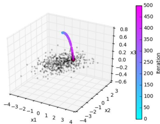
Fig. 11: Learning from a 3D input.
