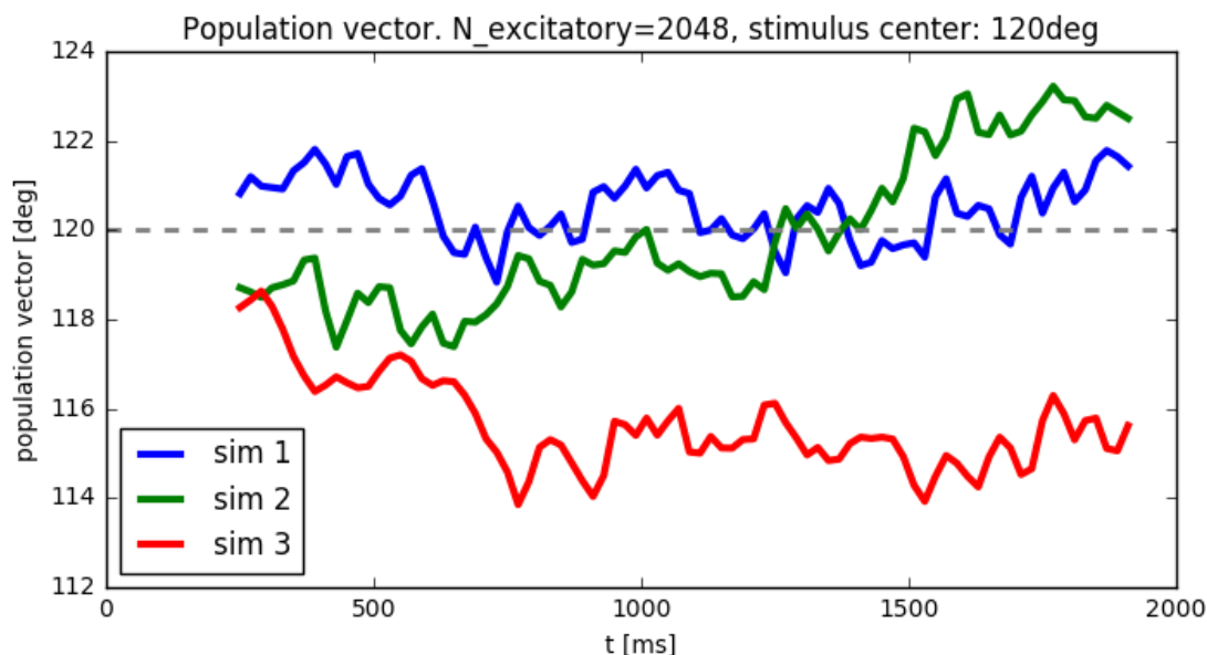
Fig. 17: Diffusion of the population vector for three different simulations.
