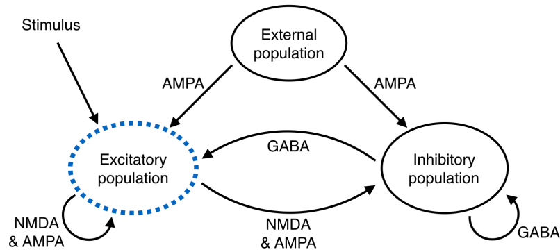
Fig. 19: Network structure. The excitatory population is divided into three subpopulations, shown in the next figure.
