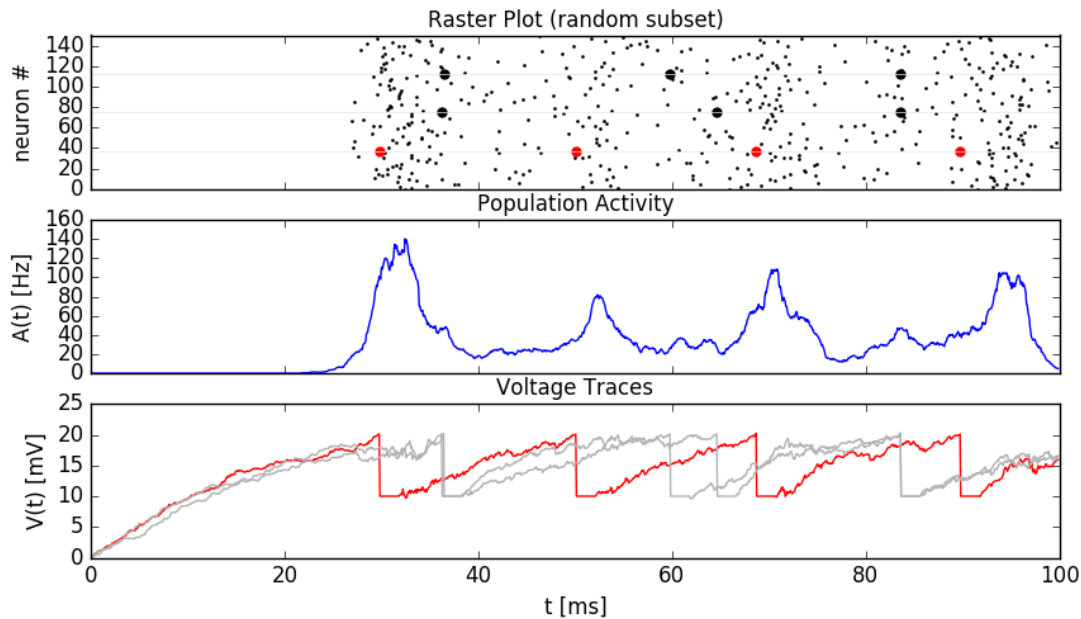
Fig. 12: Simulation result. Top: raster plot of 150 randomly selected neurons. Three spike trains are visually highlighted. Middle: time evolution of the population activity A(t) . Bottom: Membrane voltage of three neurons. The red color in the top and bottom panels identifies the same neuron.
