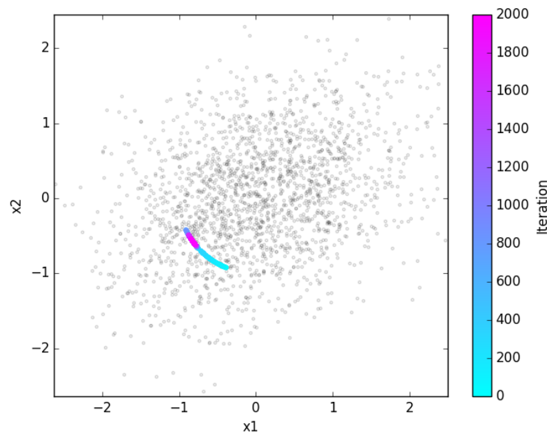
Fig. 9: Grey points: Datapoints (two presynaptic firing rates, presented sequentially in random order). Colored points: weight change under Oja's rule.
