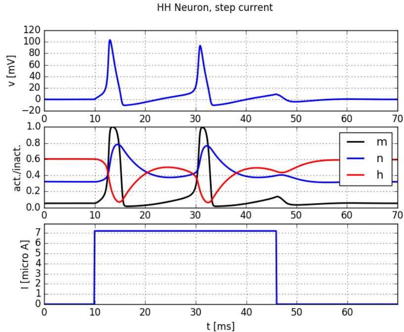
Fig. 5: Step current injection into a Hodgkin-Huxley neuron
