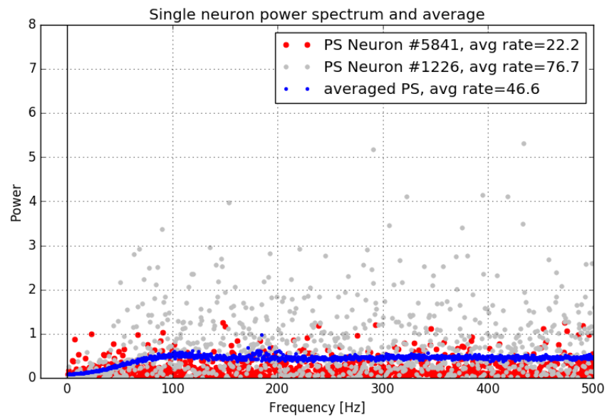
Fig. 14: Single neurons (red, grey) fire irregularly ( I ) while the population activity oscillates ( S ).
