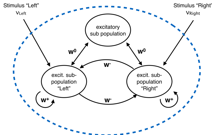
Fig. 20: Structure within the excitatory population. The “Left” and “Right” subpopulations have strong recurrent weights ( w^+ > w^0 ) and weak projections to the other ( w^- < w^0 ). All neurons receive a poisson input from an external source. Additionally, the neurons in the “Left” subpopulation receive poisson input with some rate \nu_{Left} ; the “Right” subpopulation receives a poisson input with a different rate \nu_{right} .
