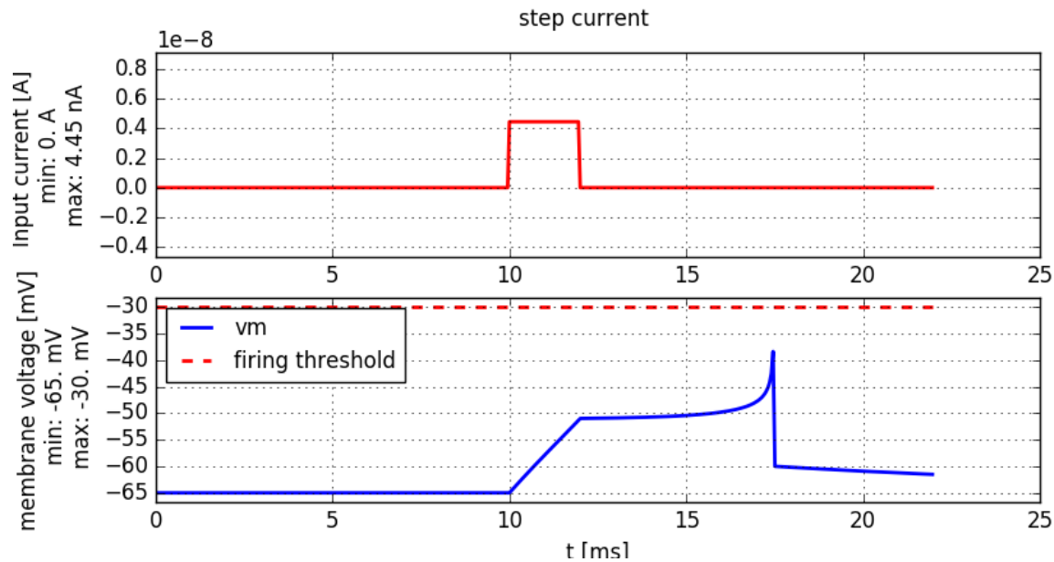
Fig. 3: A short pulse current of 2ms duration is injected into an Exponential-Integrate-and-Fire neuron. The current amplitude is just sufficient to elicit a spike.
