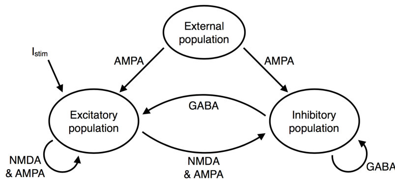
Fig. 16: Network structure. Look at Figure 18.4 in chapter 18.1 to see how the excitatory population is spatially arranged on a ring and has a specific connectivity profile. In our implementation, every excitatory neuron receives unstructured input from all inhibitory neurons and structured input from all excitatory neurons. The inhibitory neurons receive unstructured input from all excitatory and all inhibitory neurons.
