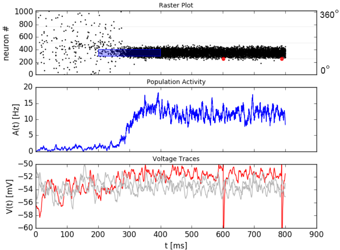
Fig. 15: Top : A weak stimulus, centered at 120deg, is applied to a subset of the excitatory population from t=200 ms to t=400 ms (blue box in top panel). This creates an activity bump in the excitatory subpopulation. The activity sustains after the end of the stimulation. The active neurons have a preferred direction close to the stimulus location. Middle : The population activity increases over time when the stimulus is applied. Bottom : Voltage traces for three selected neurons. The spikes of the red neuron are visible in the top and bottom panel.
