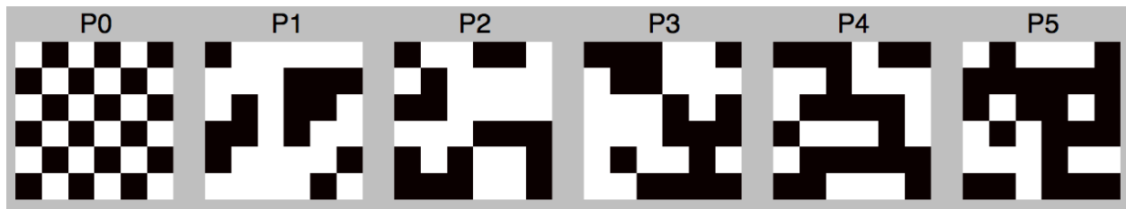
Fig. 6: Six patterns are stored in a Hopfield network.
