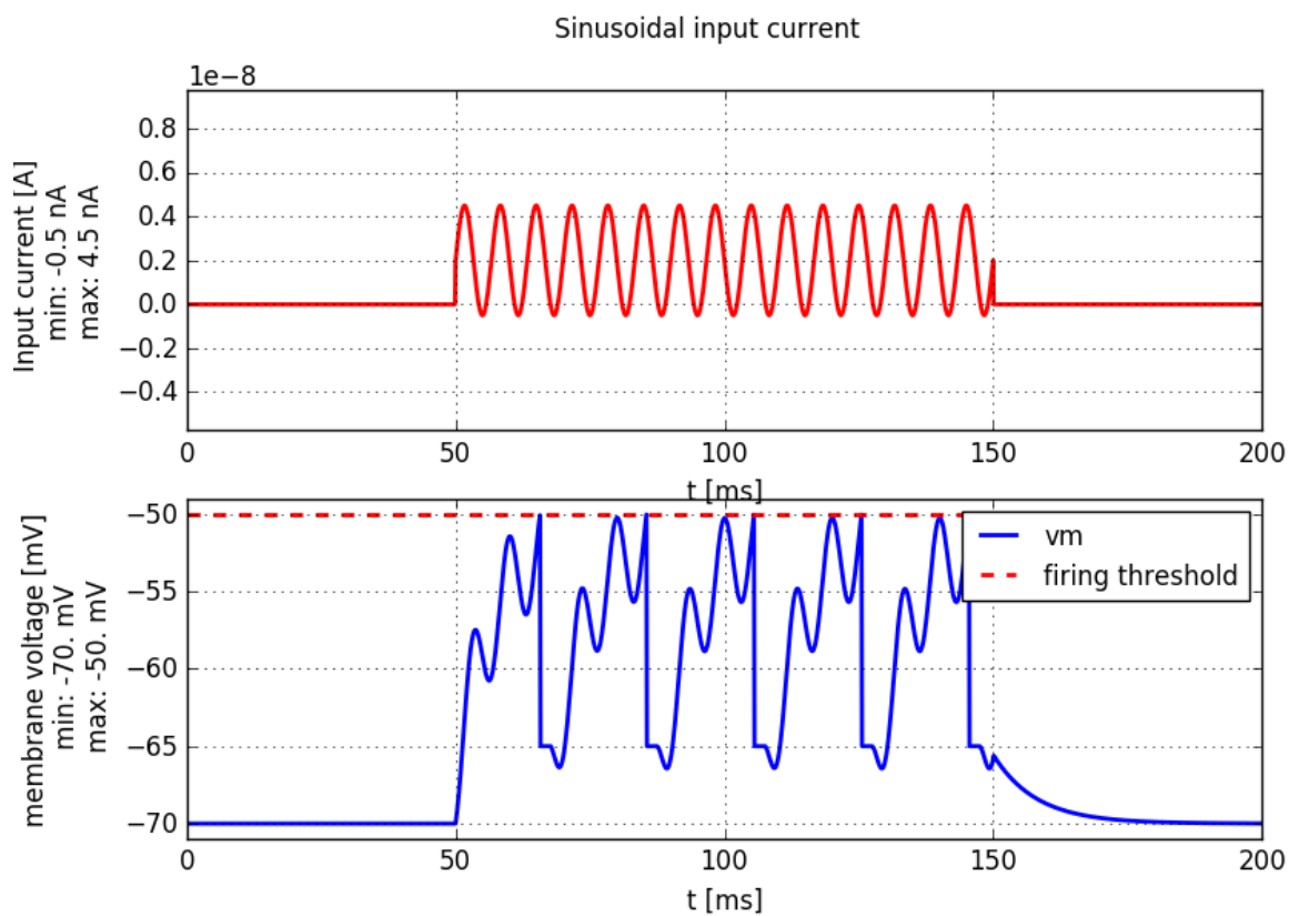
Fig. 2: Injection of a sinusoidal current into a leaky-integrate-and-fire neuron
