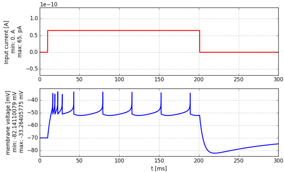
Fig. 1.4: A step-current (top panel, red) is injected into an AdEx neuron. The membrane voltage of the neuron is shown in blue (bottom panel).
